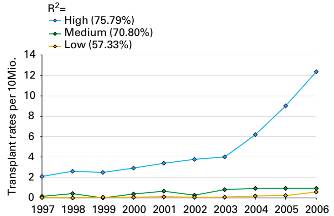
Figure 3 Evolution of cord blood HSCT in Europe from 1997 to 2006. Curves reflect means of weighted transplant rates per 10 million inhabitants according to World Bank category; high, medium and low incomes (see text) of the participating countries.
